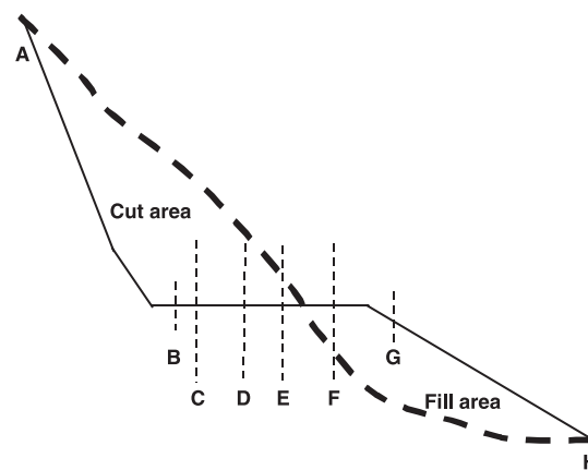
Fig. 1. Sketch of typical roadway components, showing pre- (dotted line) and post-construction (solid line) contours. AB and GH are sampled areas. BC and FG are mowed, unsampled areas. CD and EF are paved travel lanes, and DE is a mowed, vegetated median. Drawing not to scale.
