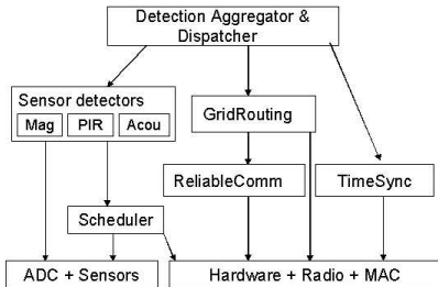
Figure 3. ExScal Op-App Tier-1 components.
