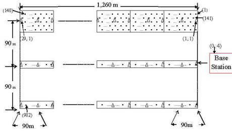
Figure 1. ExScal network topology.
