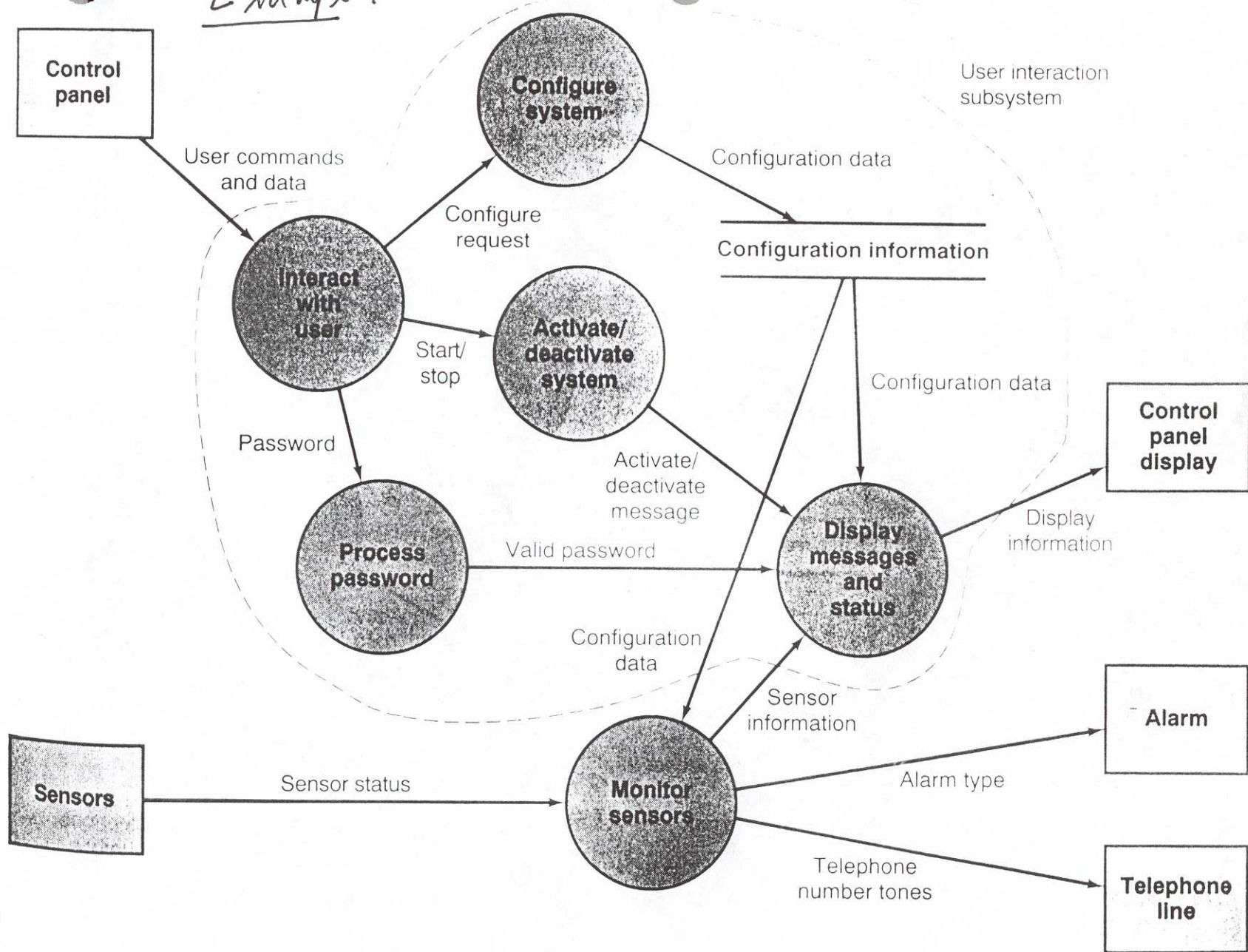
FIGURE 11.5. Level 1 DFD for SafeHome.
