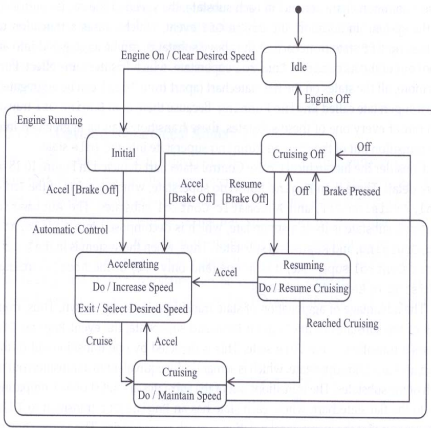
Figure 10.19 Hierarchical Cruise Control statechart with activities and exit action
