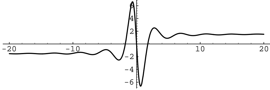
Figure 1: Graph of function f from Lemma 2.8.
