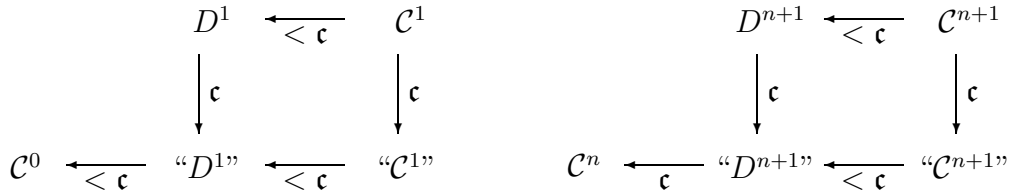
Chart 2. Values of cov operator: for n = 0 (left) and n > 0 (right).
